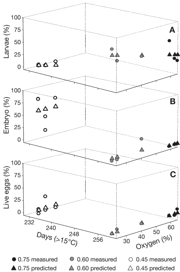
Fig. 6. Limulus polyphemus . Percentage of egg development to (A) larvae, (B) embryos, and (C) live eggs as a function of measured dissolved oxygen and interstitial temperature (expressed as degree days greater than 15°C) after 44 d across the foreshore. Circles represent measured egg development stage and triangles represent predicted egg development stage from multiple regression analysis. Fewer predicted versus measured values appear where there are multiple observations for the same level of the dependent variable
