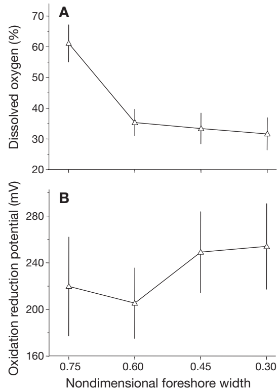
Fig. 3. (A) Dissolved oxygen and (B) oxidation reduction potential. Error bars: upper and lower 95% confidence limits
