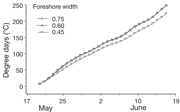
Fig. 2. Pore water temperature (°C) as a function of degree days
